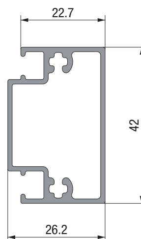
8680 0,578 Kg/m
